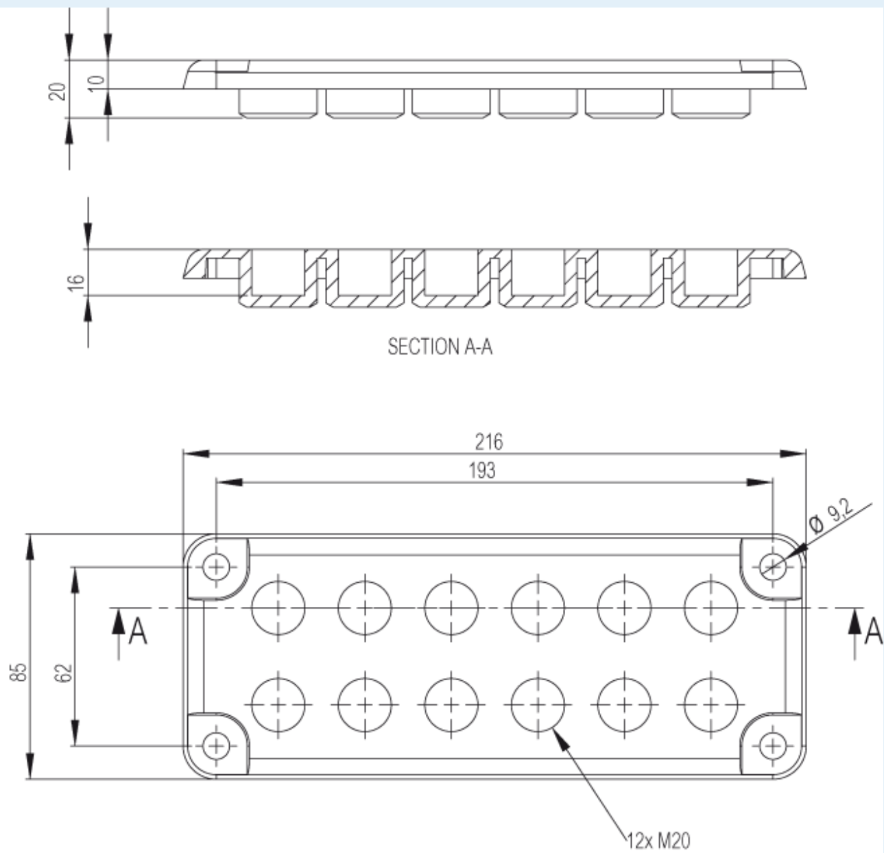
FIBOX MB 10891
