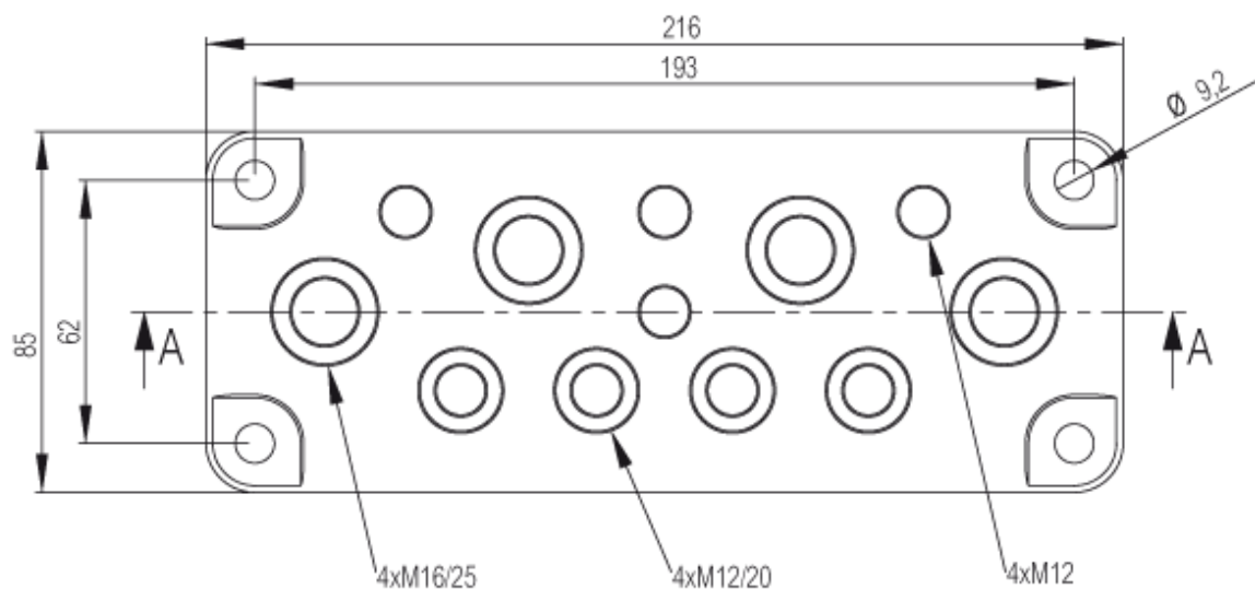
FIBOX MB 10857
